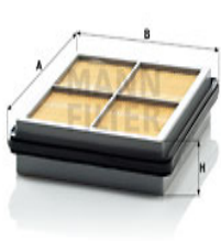
Air Filters C 2138/3 EM-30169
